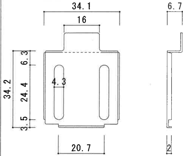
N S 126振止
